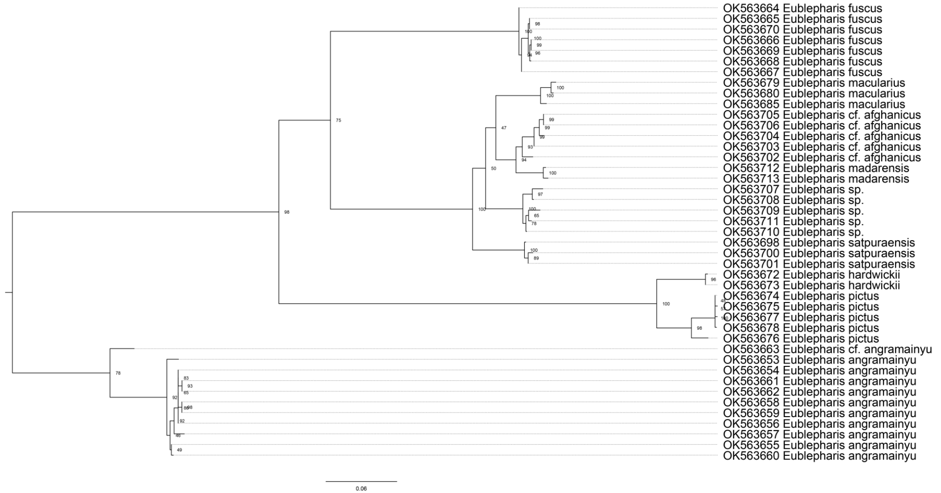
Figure S1. ML phylogeny inferred from mitochondrial ND2 gene for members of the genus Eublepharis spp.
